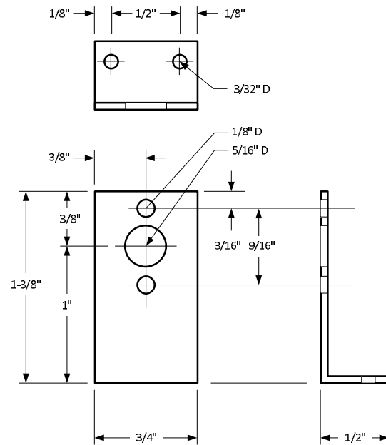
Variable Capacitor Bracket
