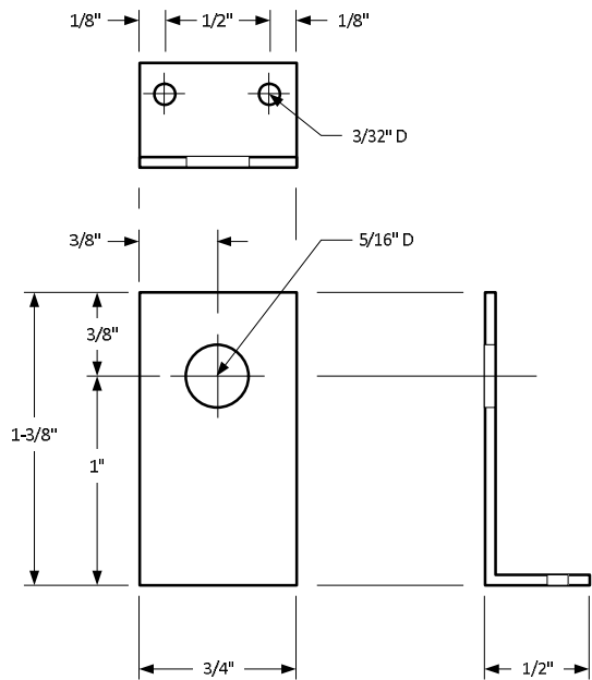
Antenna Coil Bracket
